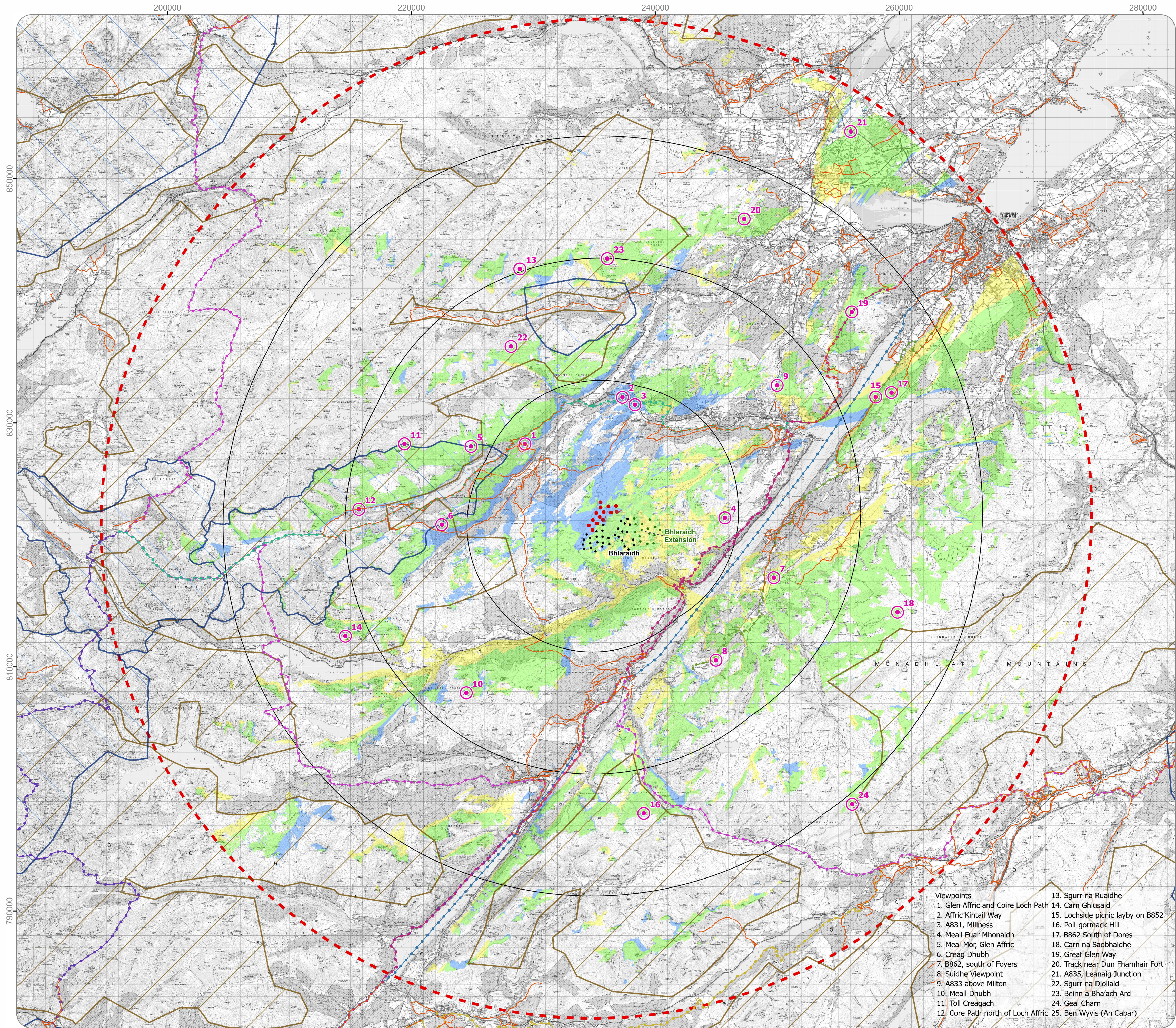
AI Figure 7.2 Cumulative ZTV with operational Bhlaraidh and consented Bhlaraidh Extension wind farms
